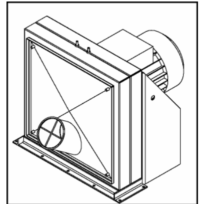
President Hammer mill type 4KSG with bottom outlet and special rotor..
