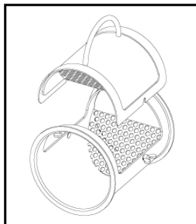
President Magnet Tube Ø150
